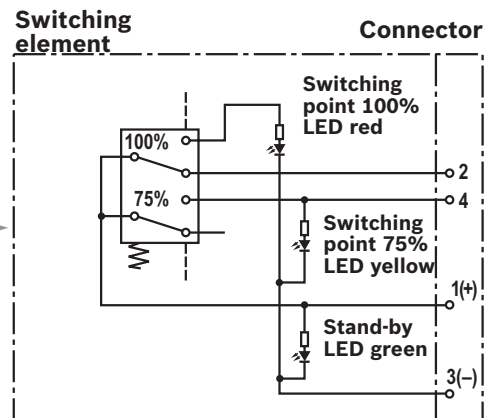
WE-2SP-M12 x 1
