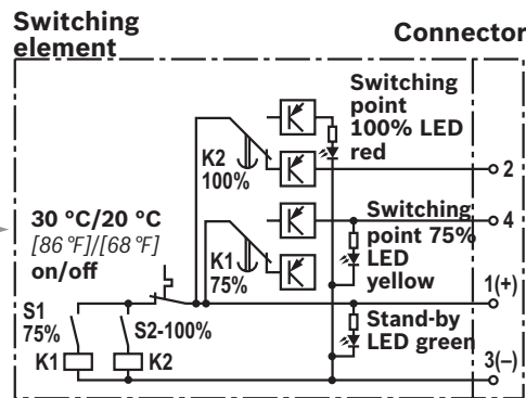
WE-2SPSU-M12 x 1
